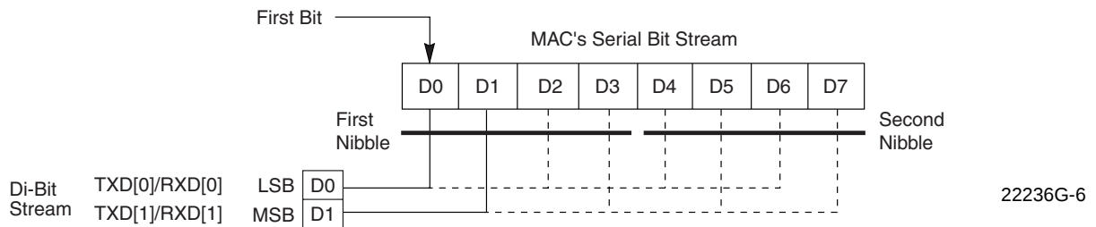
Figure 4. Bit Ordering
