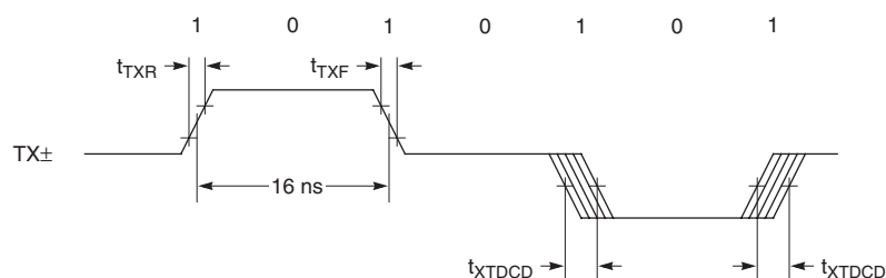
Figure 17. MLT-3 Test Waveform
