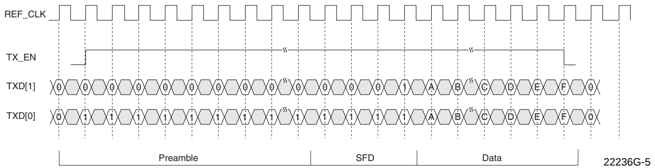
Figure 3. 100 Mbps Transmission
