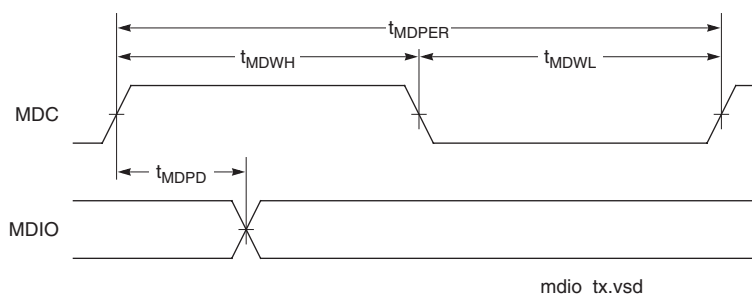
Figure 18. Management Bus Transmit Timing
