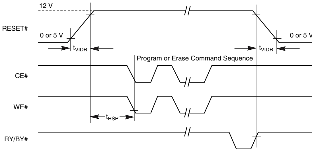
Figure 18. Temporary Sector Unprotect Timing Diagram
