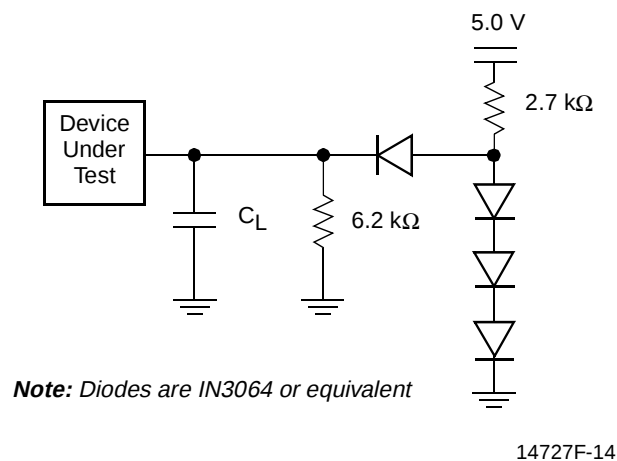
Figure 6. Test Setup
