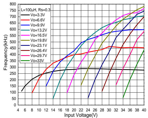
Operating Frequency vs. Input Voltage (TSOT25, R_s=0.3\Omega , L=100\mu\text{H} )
