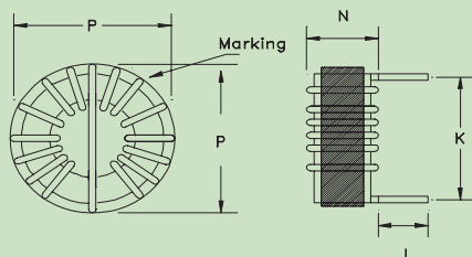
HORIZONTAL MOUNTED
