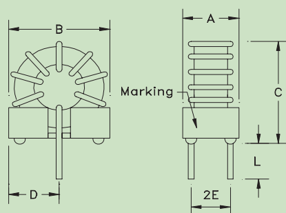
BASE MOUNTED
