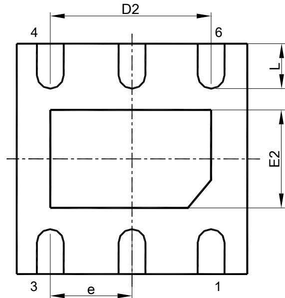
BOTTOM VIEW
