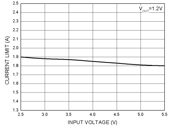
Fig. 12 Current Limit vs. Input Voltage
