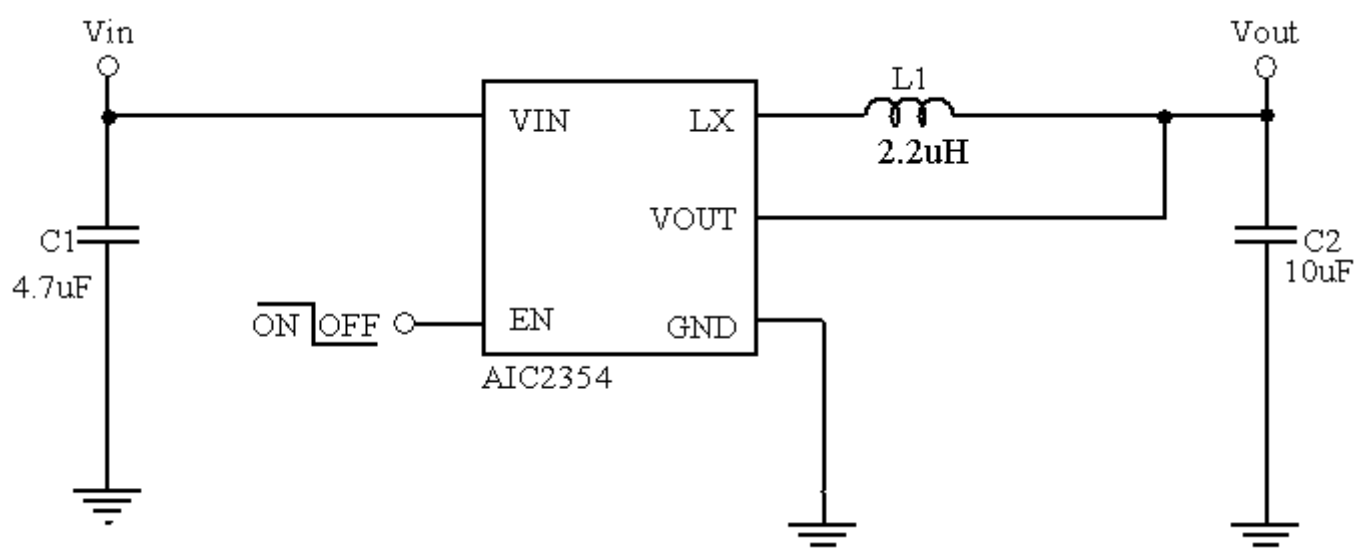
Fig. 1 Fixed Step-Down DC/DC Converter
