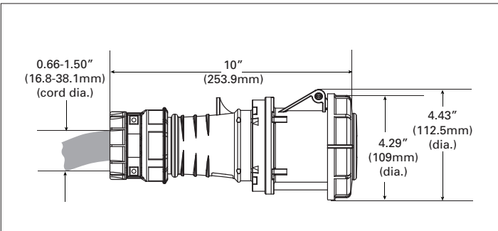
Figure 4. 60A Connectors, Side View
