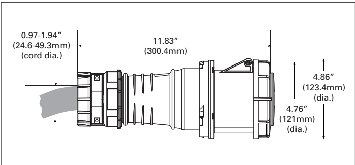
Figure 8. 100A Connectors, Side View
