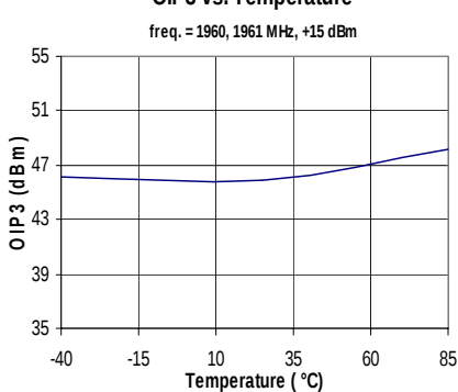
OIP3 vs. Temperature
