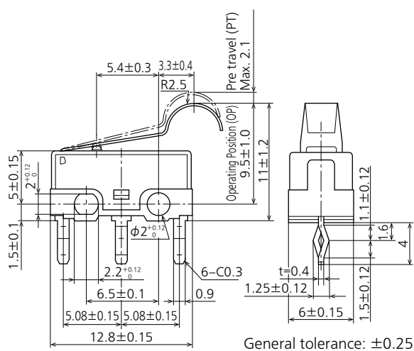
External dimensions
