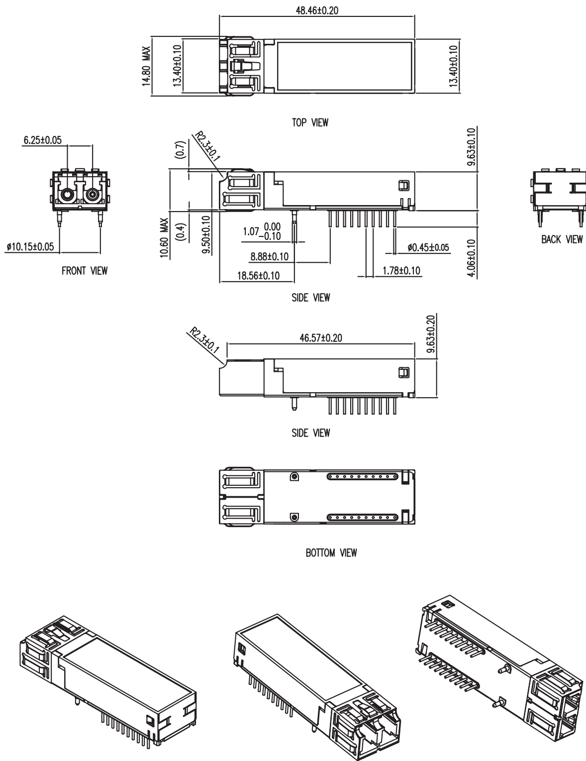
Figure 4. AFCT-5944xxZ Package Outline Drawing
