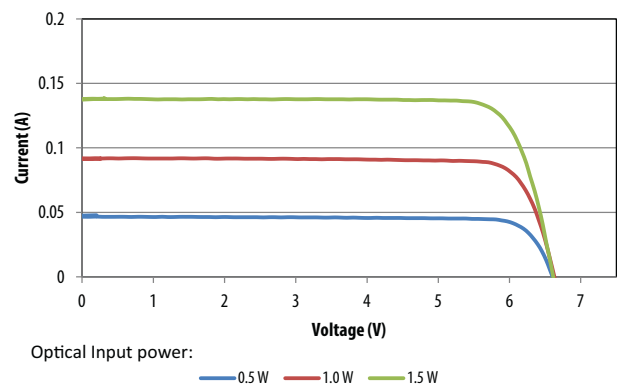
Figure 10: Output I-V Curves at 25^{\circ}\text{C} ; 1 × AFBR-POCx06L
