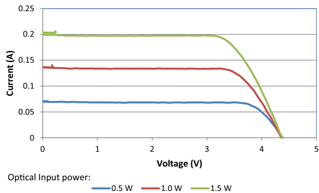
Figure 4: Output I-V Curves at 25°C; 1 × AFBR-POCx04L
