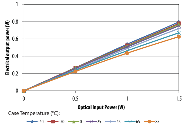
Figure 12: Electrical Output Power; 1 × AFBR-POCx06L
