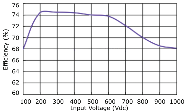
AE10-EW-S5-T Efficiency Curve Efficiency vs. Input Voltage
