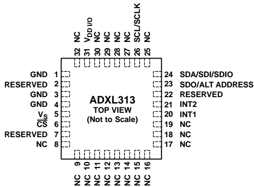
Figure 2. Pin Configuration
