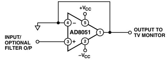
Figure 106. Recommended DAC Output Buffer Using an Op Amp
