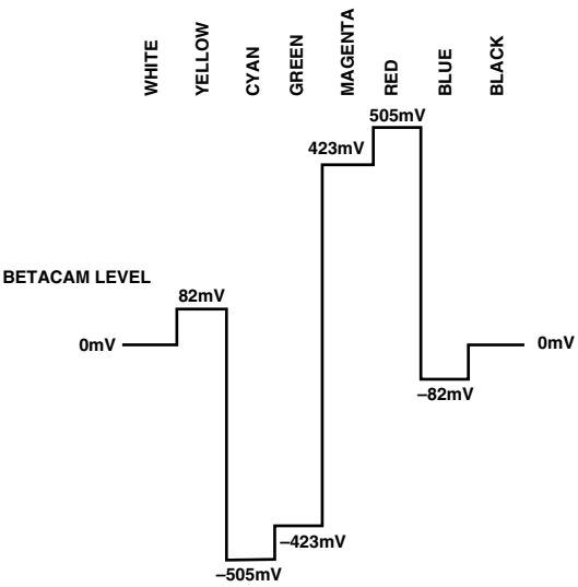
Figure 124. NTSC 100% Color Bars No Pedestal V Levels
