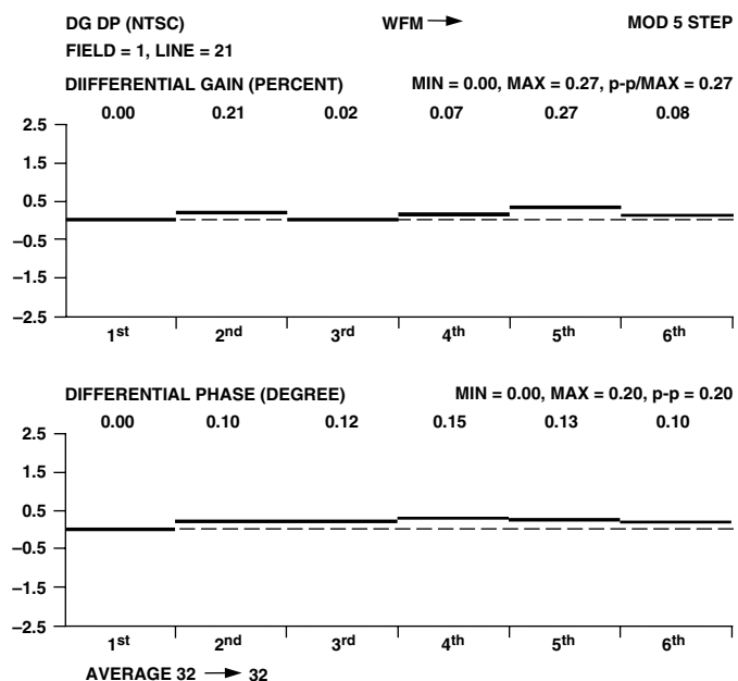
Figure 135. NTSC DG DP Measurement
