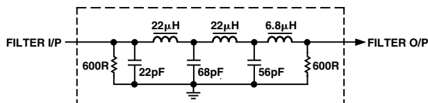
Figure 100. Output Filter for 2× Oversampling Mode
