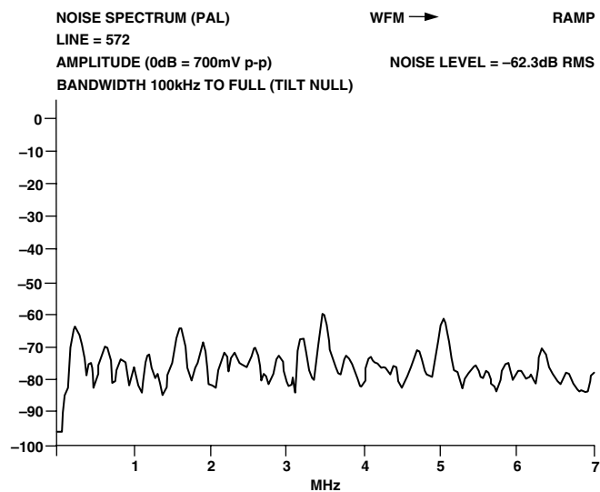
Figure 146. PAL Noise Spectrum: Ramp
