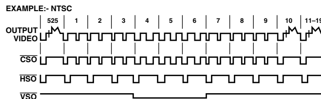
Figure 31. \overline{\text{CSO}} , \overline{\text{HSO}} , \overline{\text{VSO}} Timing Diagram
