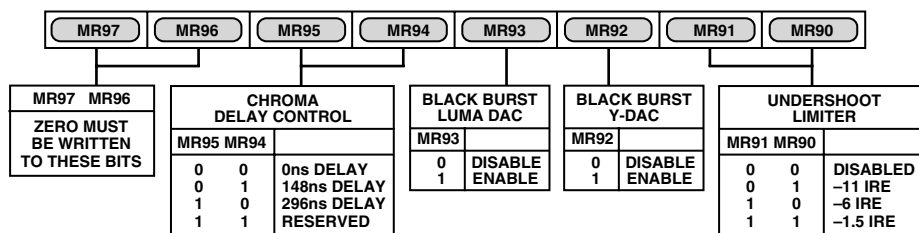
Figure 65. Mode Register 9, MR9
