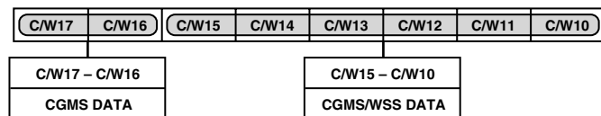
Figure 76. CGMS_WSS Register 1
