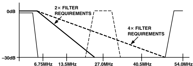
Figure 35b. Output Filter Requirements in 4× Oversampling Mode
