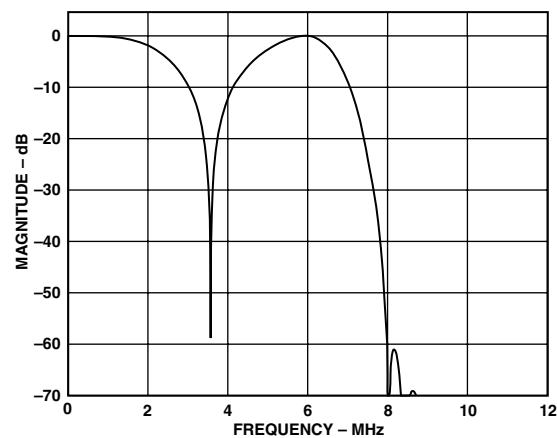
Figure 13. NTSC Notch Luma Filter
