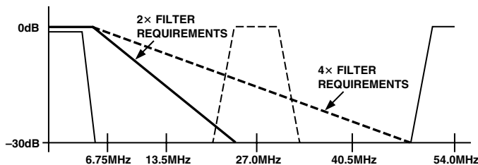
Figure 8. Output Filter Requirements in 2× and 4× Oversampling Mode
