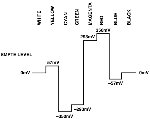
Figure 126. PAL 100% Color Bars V Levels
