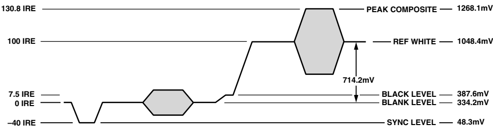
Figure 107. NTSC Composite Video Levels
