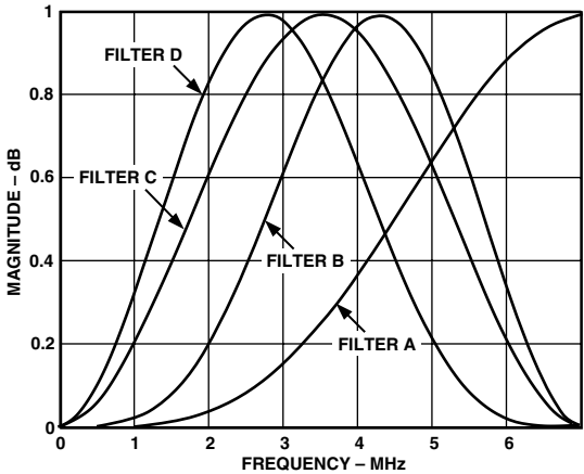
Figure 87. Filter Response of Filters Selectable
