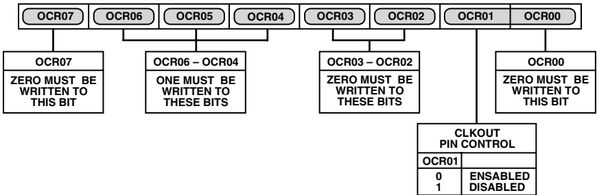
Figure 93. Mode Register 10 (MR10)
