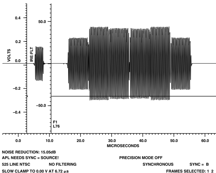
Figure 132. 100/7.5/75/7.5 NTSC Color Bars Chrominance
