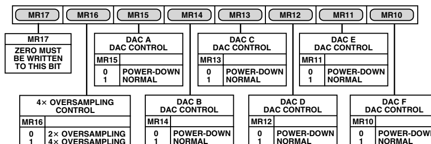
Figure 56. Mode Register 1, MR1
