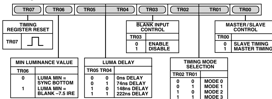
Figure 66. Timing Register 0
