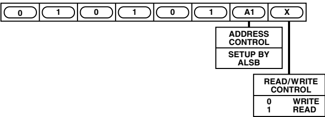
Figure 51. Slave Address
