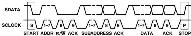
Figure 52. Bus Data Transfer
