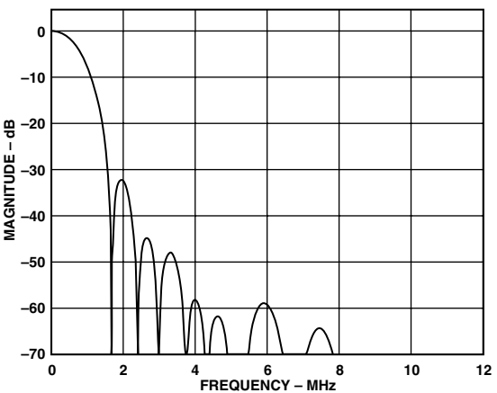
Figure 26. Chroma CIF Filter
