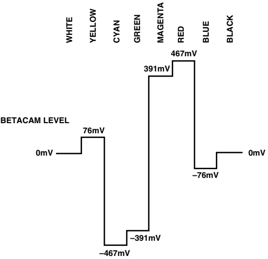
Figure 125. NTSC 100% Color Bars with Pedestal V
