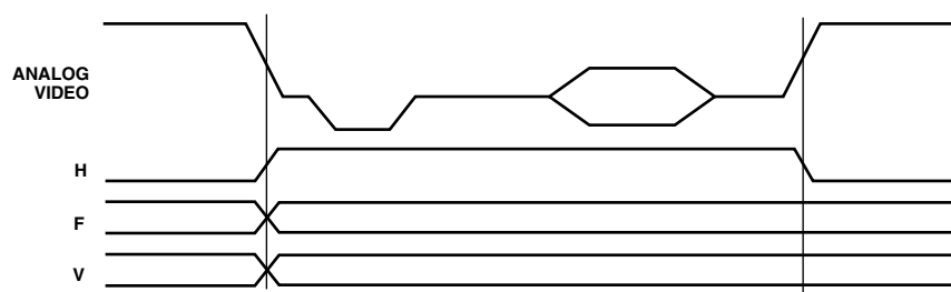
Figure 41. Timing Mode 0 Data Transitions, Master Mode
