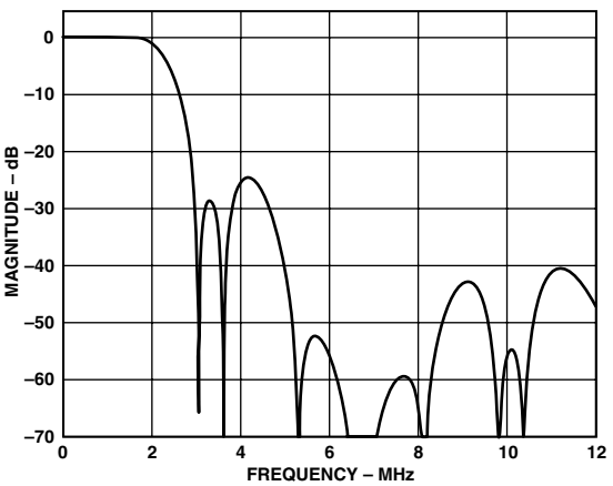
Figure 25. Chroma 2 MHz Low-Pass Filter
