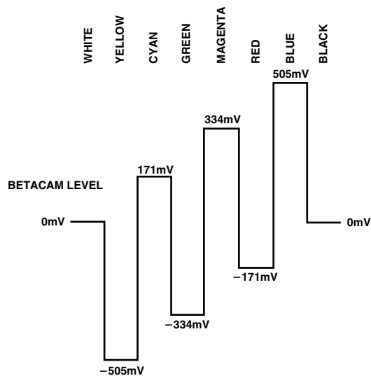
Figure 121. NTSC 100% Color Bars No Pedestal U Levels
