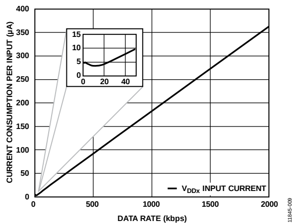
Figure 13. Current Consumption per Input vs. Data Rate for 3.3 V, \text{EN}_x = \text{Low Operation}
