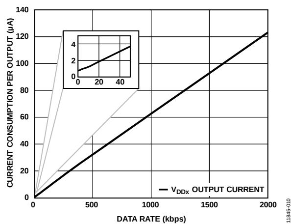
Figure 14. Current Consumption per Output vs. Data Rate for 3.3 V, \text{EN}_x = \text{Low Operation}
