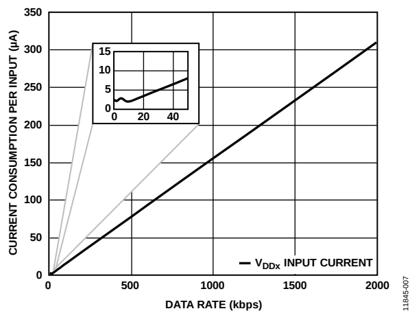
Figure 11. Current Consumption per Input vs. Data Rate for 2.5 V, \text{EN}_x = \text{Low Operation}
