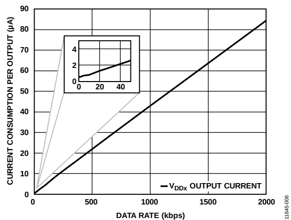
Figure 12. Current Consumption per Output vs. Data Rate for 2.5 V, \text{EN}_x = \text{Low Operation}
