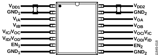
Figure 29. Recommended Printed Circuit Board Layout, QSO
