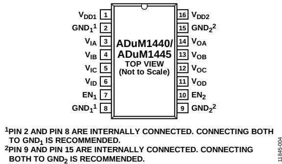
Figure 5. ADuM1440/ADuM1445 QSO Pin Configuration
