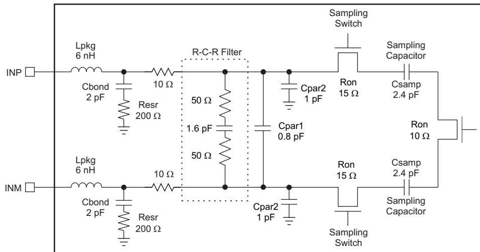
Figure 38. Input Stage
