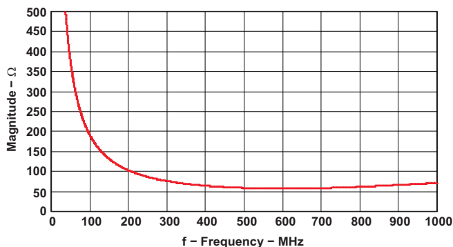
Figure 41. Input Impedance, Z_i
