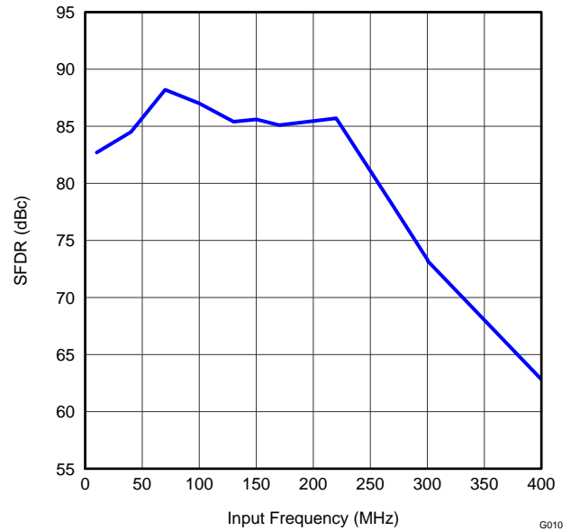
Figure 22. SPURIOUS-FREE DYNAMIC RANGE vs INPUT FREQUENCY G010
