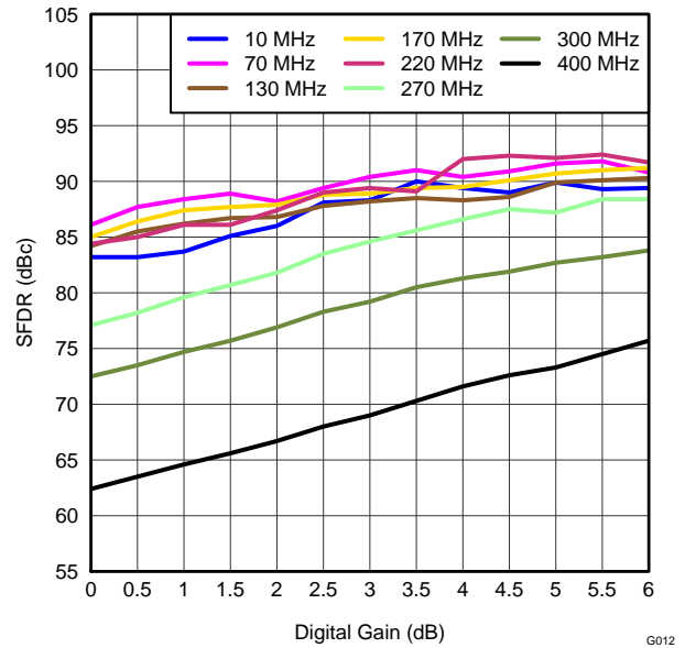
Figure 24. SPURIOUS-FREE DYNAMIC RANGE vs GAIN AND INPUT FREQUENCY G012
