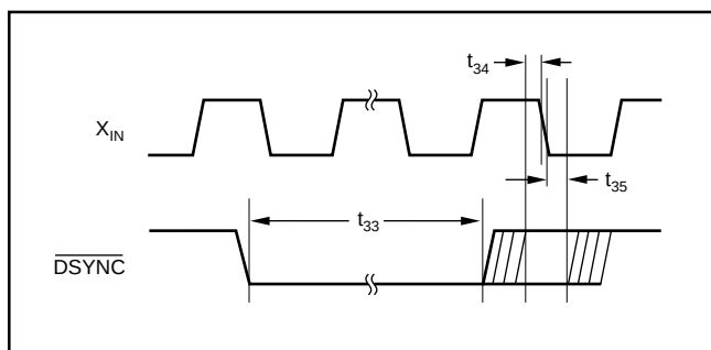
FIGURE 22. \overline{\text{DSYNC}} to X_{\text{IN}} Timing for Synchronizing Mutliple ADS1210/11s.
