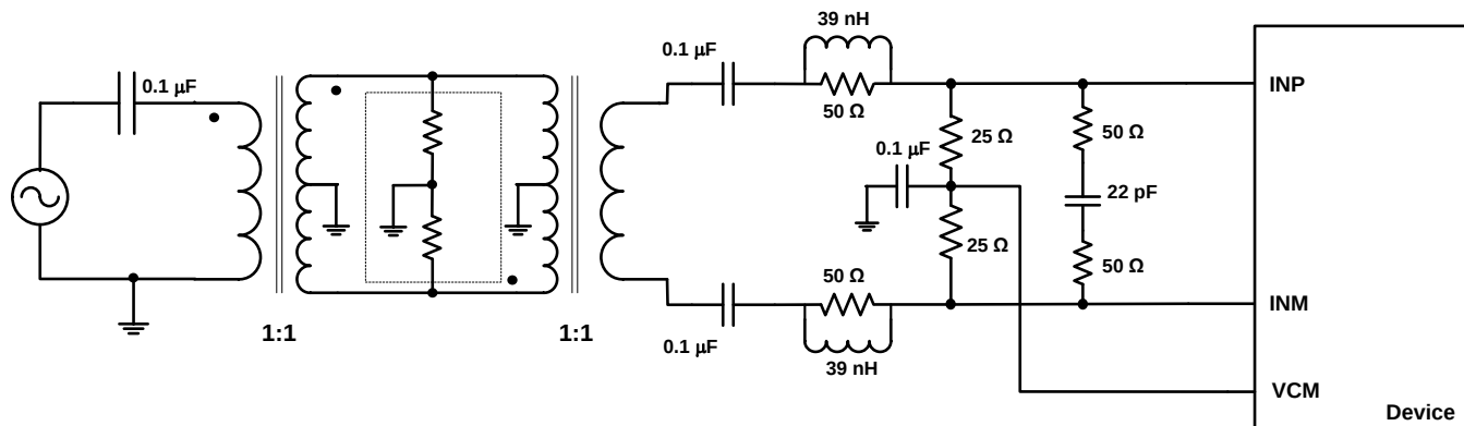
Figure 177. Driving Circuit for Low Input Frequencies
