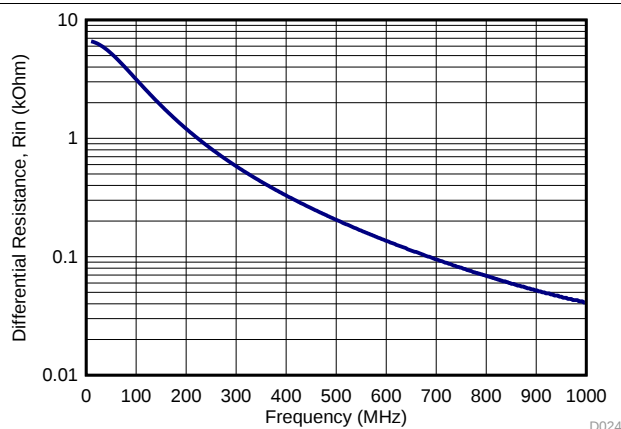
Figure 175. Differential Input Resistance (R IN )
