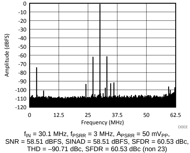
Figure 126. Power-Supply Rejection Ratio Spectrum
