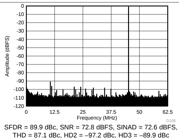
Figure 99. FFT for 170-MHz Input Signal (Dither Off)
