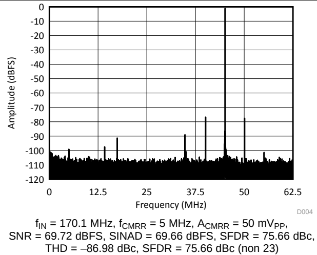
Figure 128. Common-Mode Rejection Ratio Spectrum
