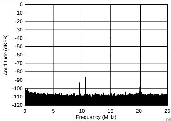
Figure 34. FFT for 70-MHz Input Signal (Dither On)
