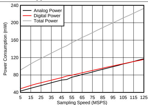
Figure 129. Power vs Sampling Frequency (One-Wire Mode)
