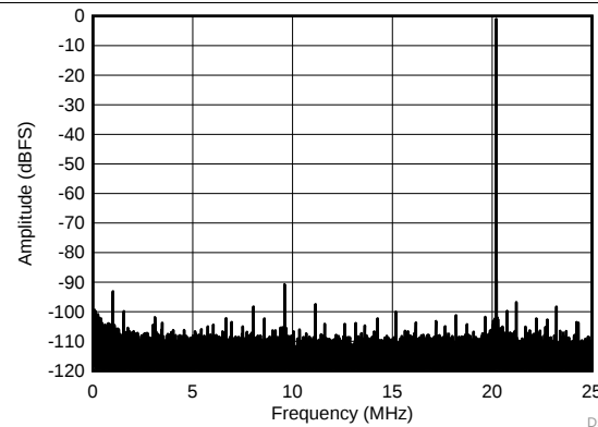
Figure 35. FFT for 70-MHz Input Signal (Dither Off)
