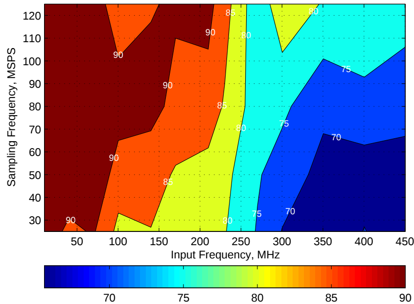
Figure 130. Spurious-Free Dynamic Range (SFDR)
