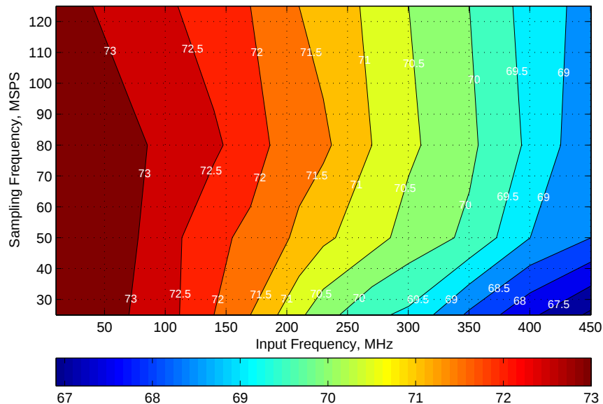
Figure 131. Signal-to-Noise Ratio (SNR)
