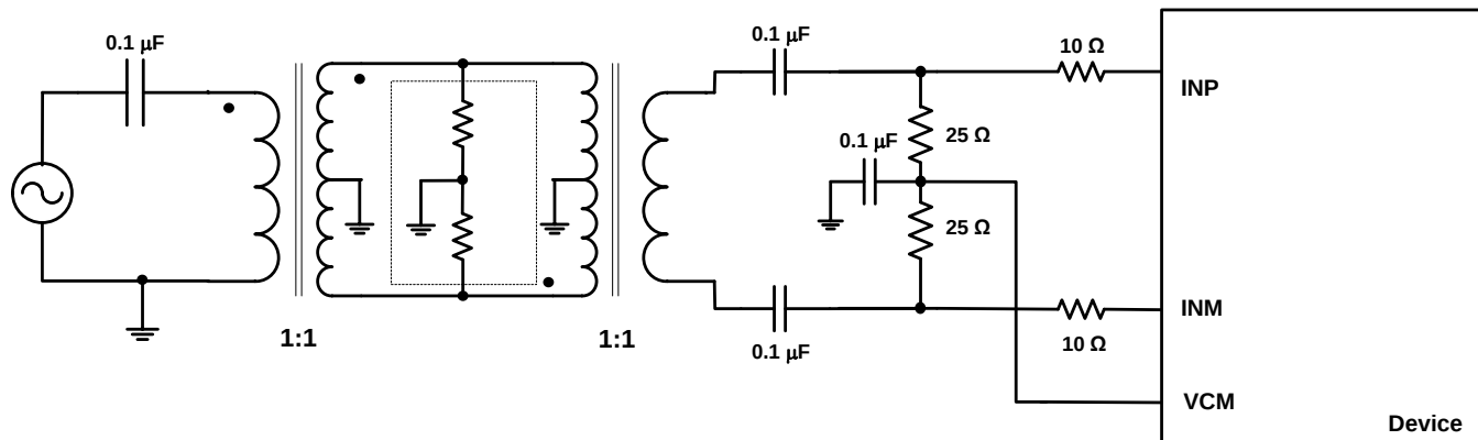
Figure 181. Driving Circuit for High input Frequencies ( f_{IN} > 230 MHz)
