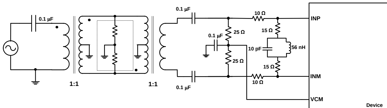
Figure 179. Driving Circuit for Mid-Range Input Frequencies ( 100 \text{ MHz} < f_{\text{IN}} < 230 \text{ MHz} )
