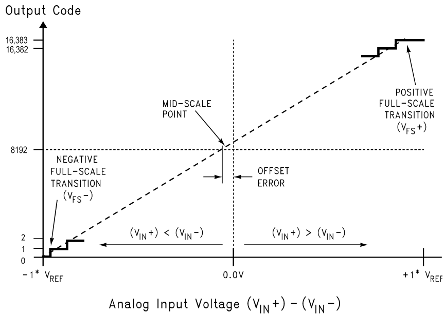
Figure 4. Transfer Characteristic
