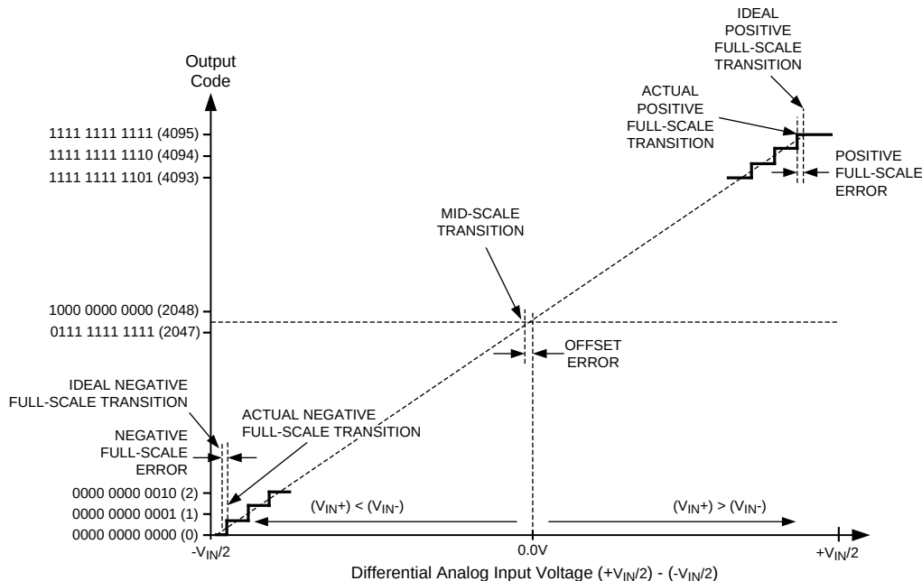
Figure 4-2. Input / Output Transfer Characteristic
