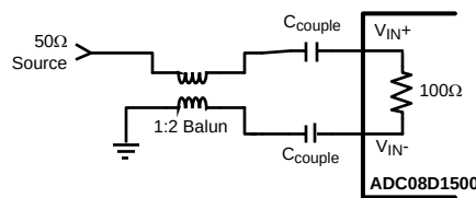
Figure 37. Single-Ended to Differential Signal Conversion Using a Balun
