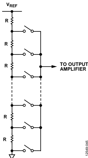
Figure 42. Simplified Resistor String Structure
