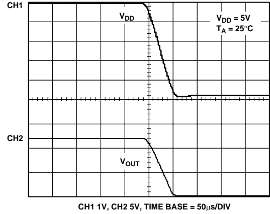
Figure 25. V DD vs. V OUT
