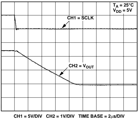
Figure 23. Half-Scale Settling Time
