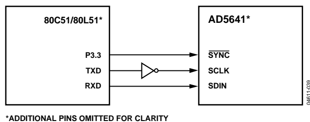
Figure 40. AD5641 to 80C51/80L51 Interface
