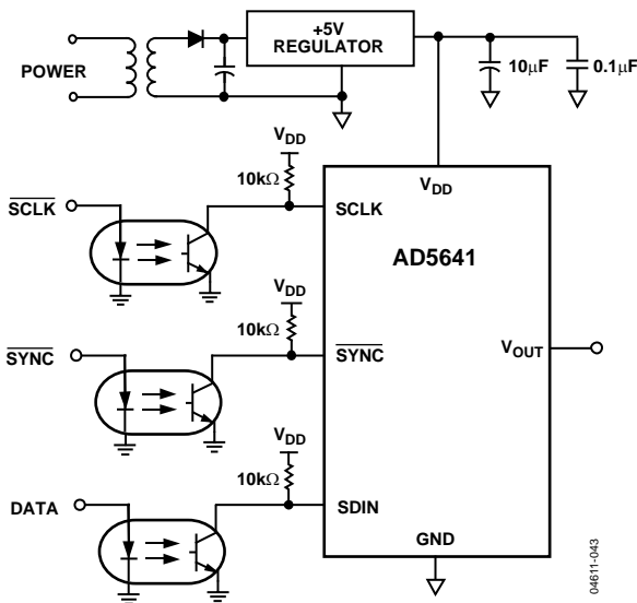
Figure 44. AD5641 with an Opto-Isolated Interface
