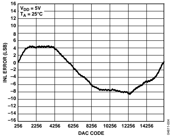
Figure 4. Typical INL
