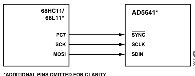
Figure 38. AD5641 to 68HC11/68L11 Interface
