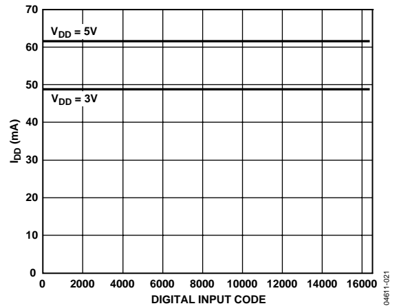
Figure 21. Supply Current vs. Digital Input Code
