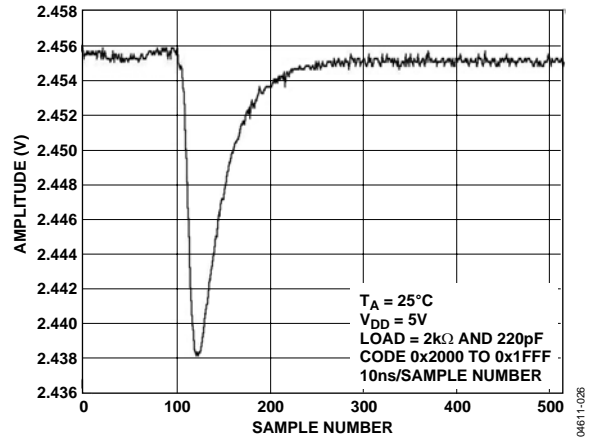
Figure 26. Digital-to-Analog Glitch Energy
