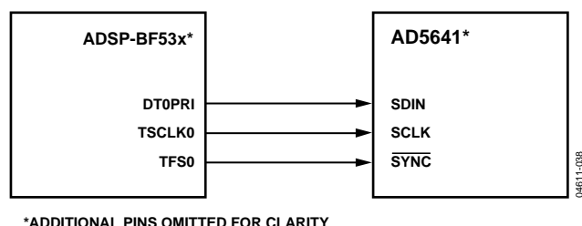
Figure 39. AD5641 to Blackfin ADSP-BF53x Interface
