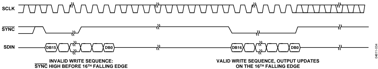
Figure 35. SYNC Interrupt Facility
