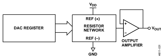
Figure 32. DAC Architecture
