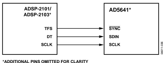
Figure 37. AD5641 to ADSP-2101/ADSP-2103 Interface
