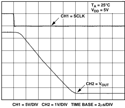
Figure 22. Full-Scale Settling Time
