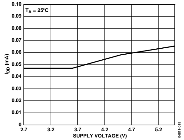
Figure 19. Supply Current vs. Supply Voltage at 25°C
