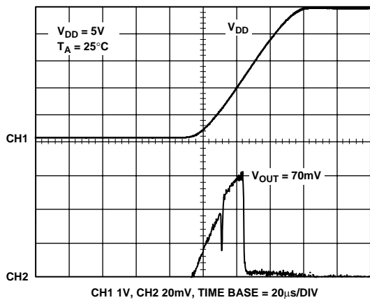
Figure 24. Power-On Reset to 0V
