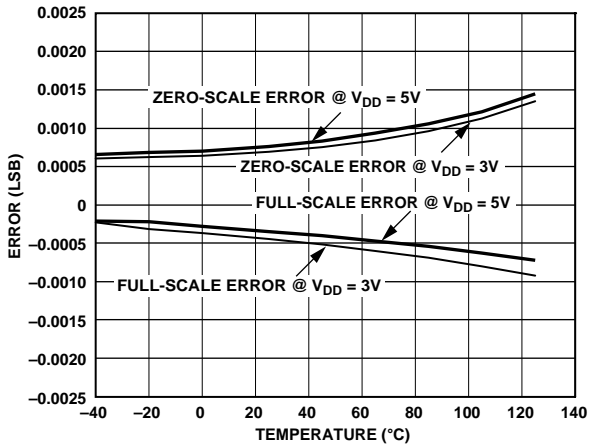
Figure 10. Zero-Code/Full-Scale Error vs. Temperature (3 V/5 V)
