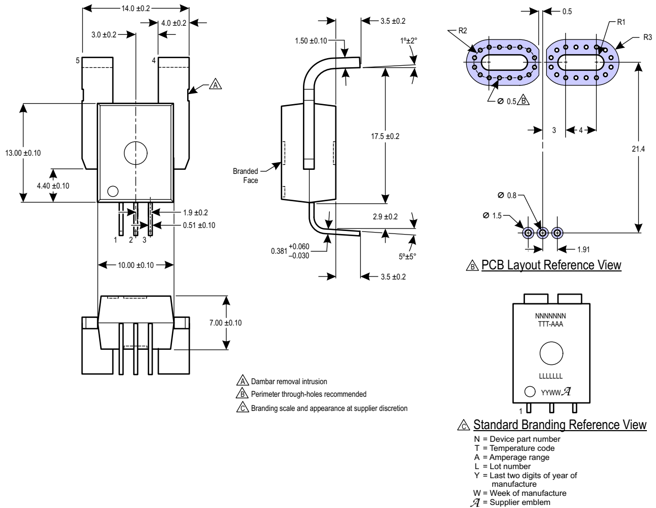
Figure 9: Package CB, 5-Pin, Leadform PFF
