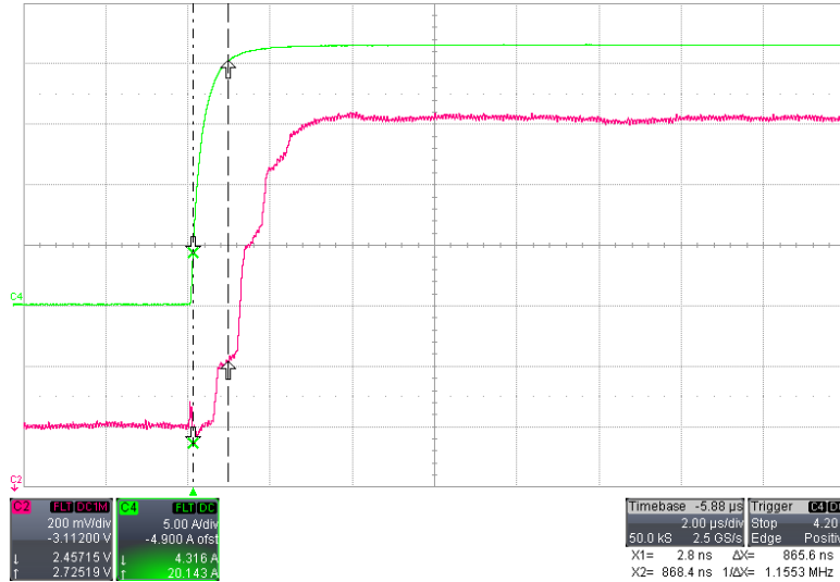
Figure 11: Propagation Delay from 20%-20% (input to output): 110 G excitation signal with rise time 10%-90% = 700 ns, Input = C4 \times 5 G/A (green), V OUT = C2 (red), no C L or R L , C BY = 0.1 \mu F
