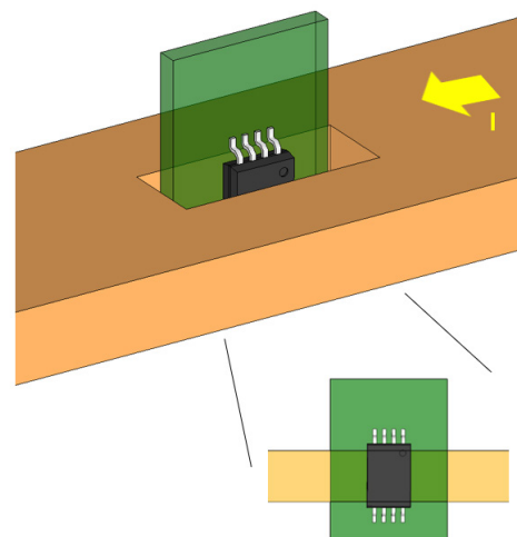
Figure 22: Vertical Slit Busbar Design
