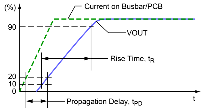
Figure 15: Propagation Delay ( t_{PD} ) and Rise Time ( t_r )
