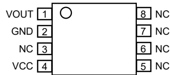
Figure 4: Pinout Diagram
