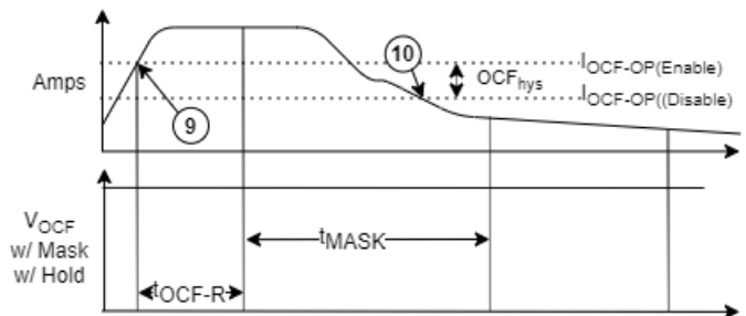
Figure 13: Fault Condition Clearing Before Mask Time Is Reached
