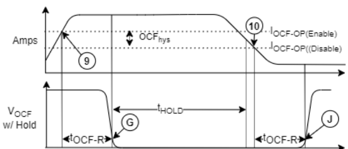
Figure 14: Fault Hold with Clear Fault After Hold Time
