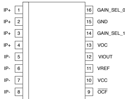
Figure 2: MC Pinout Diagram
