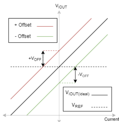
Figure 6: Offset ( V_{OFF} ) Between V_{IOUT} and V_{REF}
