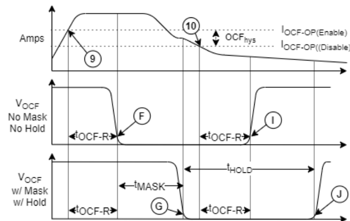
Figure 12: General Fault Timing. Note: the MASK and HOLD functionality are independent of each other
