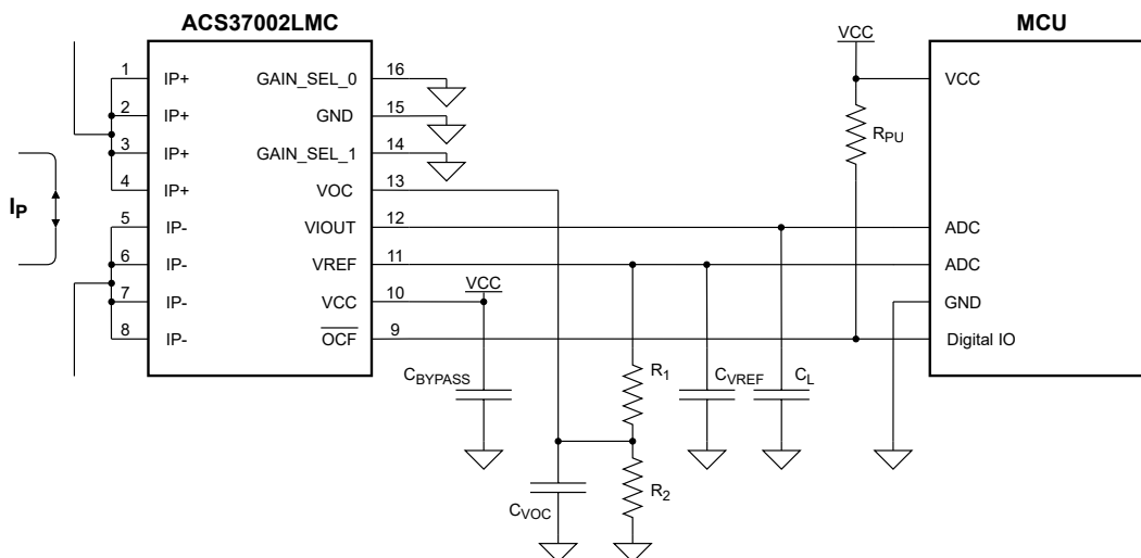
Figure 1: Typical Bidirectional Application For more application circuits, refer to the Application and Theory section
