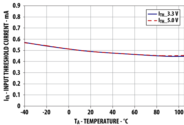
Figure 5. Input Threshold Current vs. Temperature
