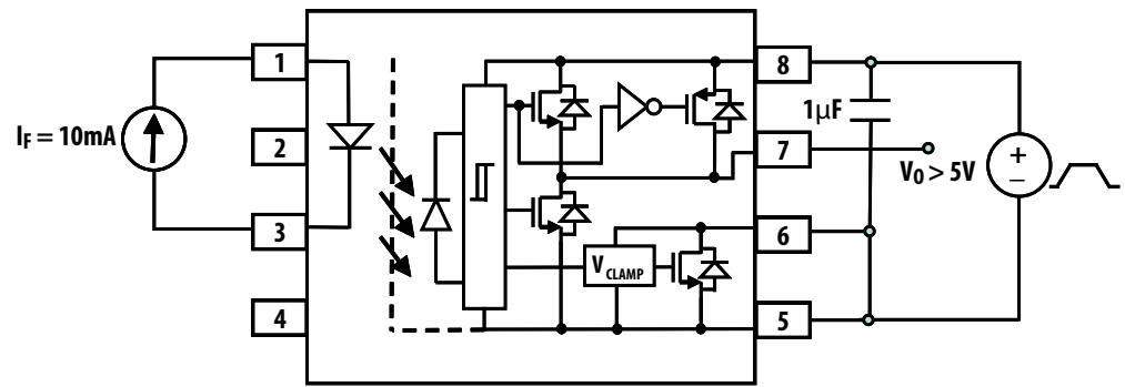
Figure 30. UVLO test circuit.
