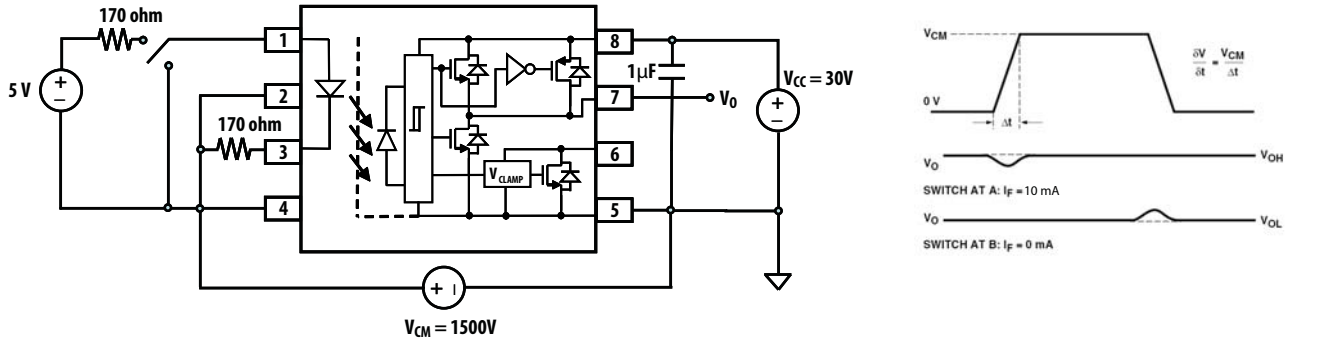
Figure 32. CMR test circuit with split resistors network and waveforms.
