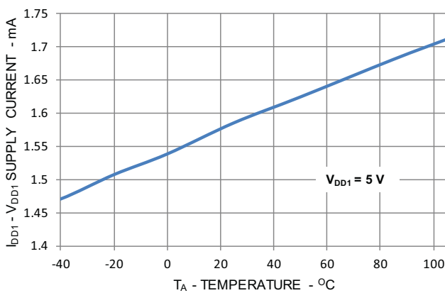
Figure 15 I_{DD1} vs. Temperature
