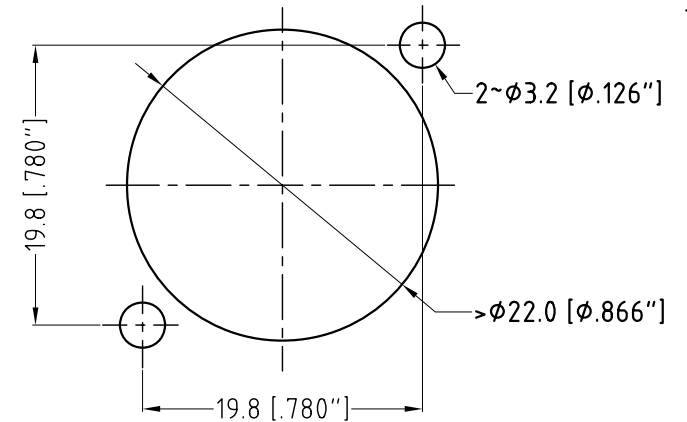
PANEL CUT OUT REAR VIEW
