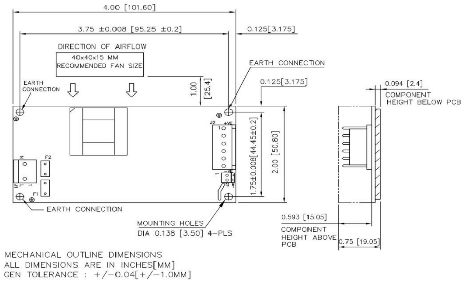
Mechanical Drawing – Option 2
