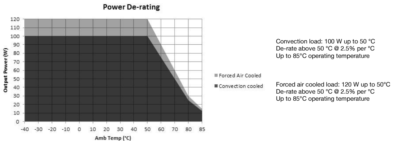
Figure 1. Derating Curve
