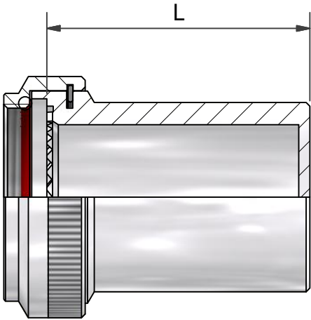
100P670-17-1-C NO ATTACHMENT VERSION
