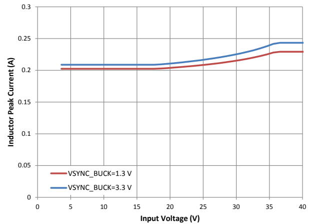
Figure 15: Typical Peak Inductor Current versus Input Voltage for 0.18 A Output Current and 10 \mu\text{H} Inductor
