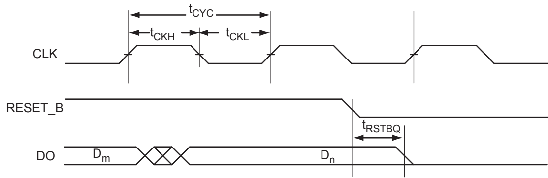
Figure 2-49 • RAM Reset
