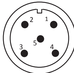
5- Pin M12 Connector Pin Out
