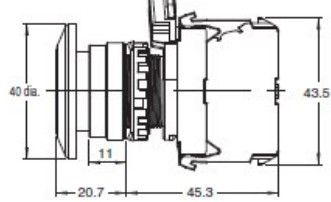
A22N[]-MM[]-[]A-P[]-[]
