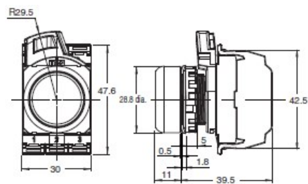
A22NN-RN[]-N[]A-P[]-NN
