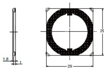
Reinforcement Plate
