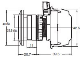
A22N[]-MM[]-[]A-P[]-[]
