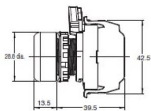
A22NN-RN[]-U[]A-P[]-NN
