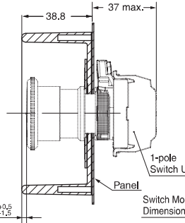
Push-in Plus Terminal Block Type Mounting a 1-pole Switch Unit
