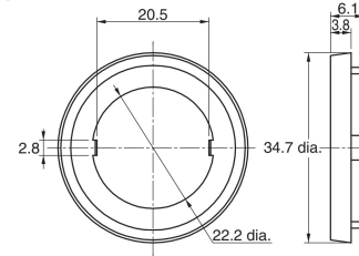
30-dia. Resin Attachment A22Z-A30
