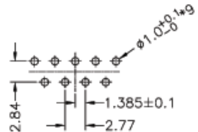
9 Pin Male Connector PCB Pin Layout Scale 2:1
