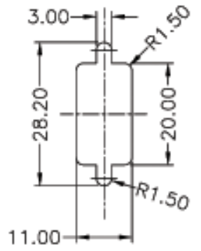
Recommended Panel Cut-Out 建議挖孔尺寸
