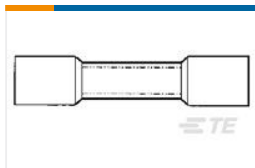
TE Part #55845-1 #8 PRE-INSUL SEALED SPLICE
