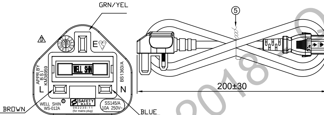
BS 1363 UK10 (10A FUSE)
