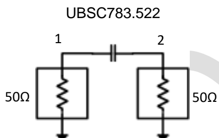
Schematic of 22nF UBSC in transmission mode
