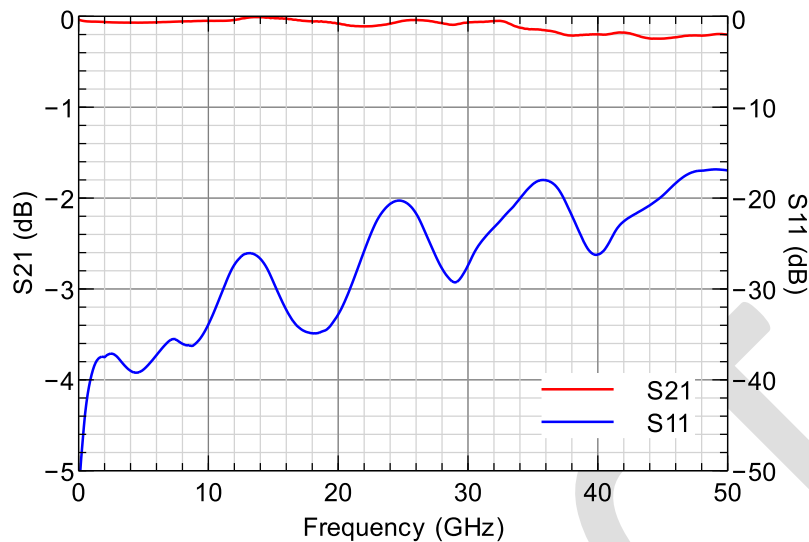
Figure 2 - 22nF ULSC Measured results (module of S-parameters)
