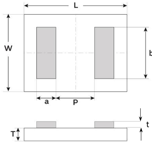
Figure 9 - Package outline drawing
