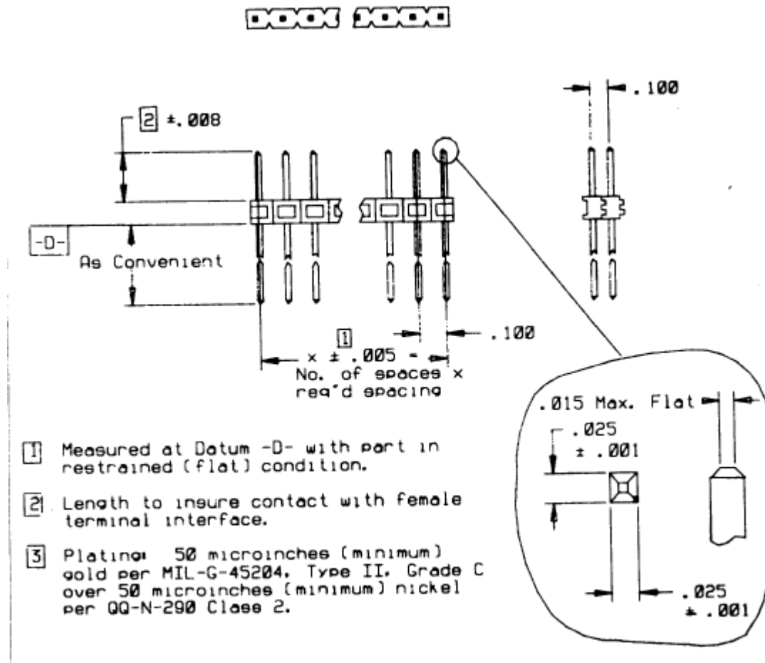
FIGURE 2- MATING HEADER
