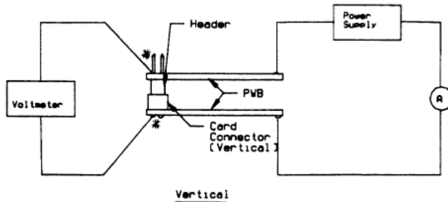
FIGURE 1 - CONTACT RESISTANCE
