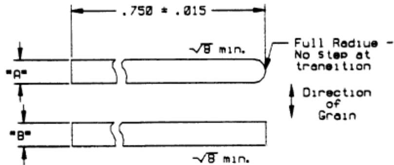
Dimensions - Inch
