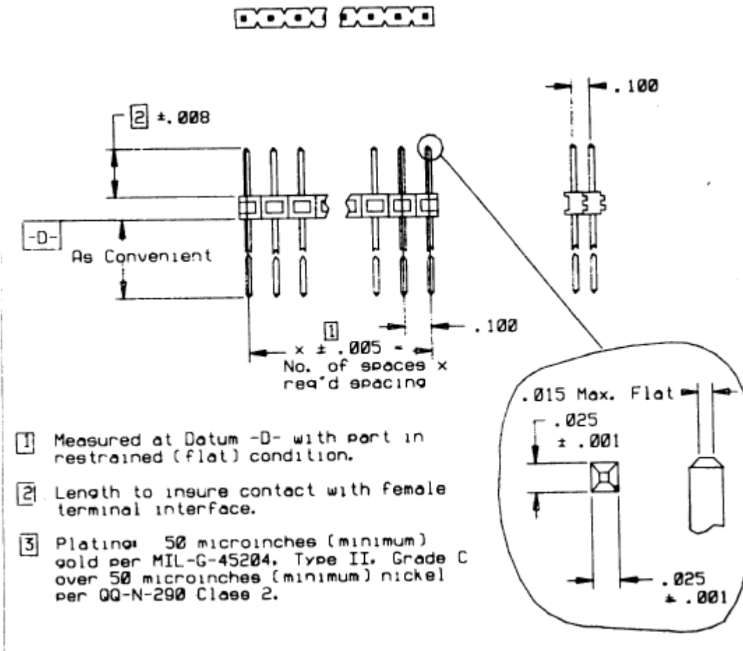
FIGURE 2- MATING HEADER
