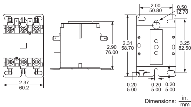
Figure 3: Type DPA, 2 and 3 Pole 20–40 Full Load Amperes
