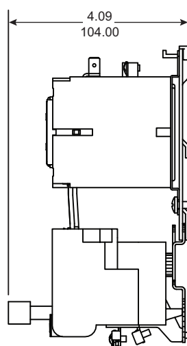
Figure 7: Approximate Dimensions
