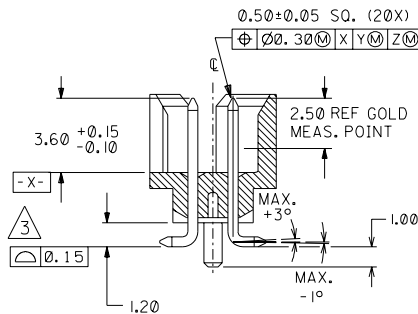
SECTION G-G
