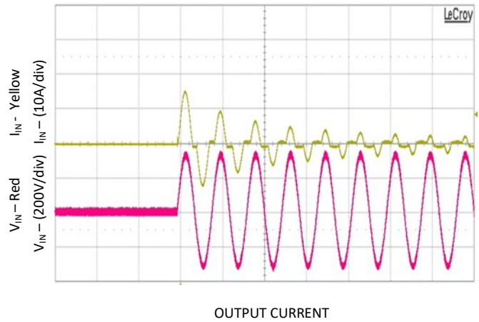
Figure 2. Inrush current V_{IN} = 230V_{AC} , 0°C phase angle
