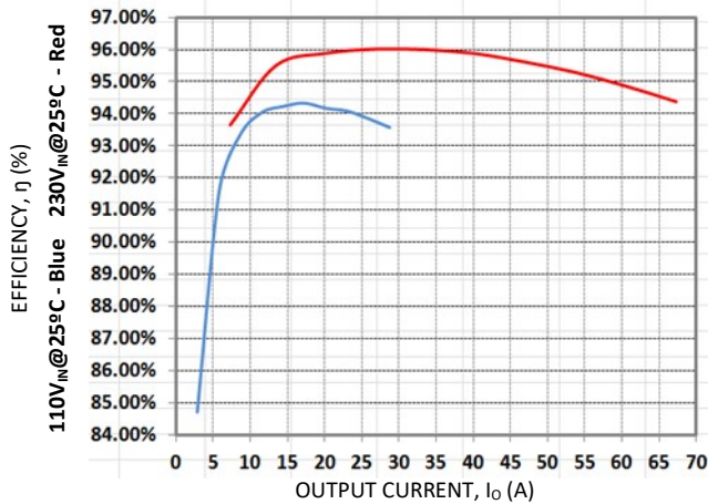
Figure 1. Rectifier Efficiency versus Output Current.
