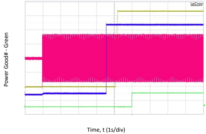
Figure 14. Turn-ON at full load V_{IN} = 230V_{AC} .
