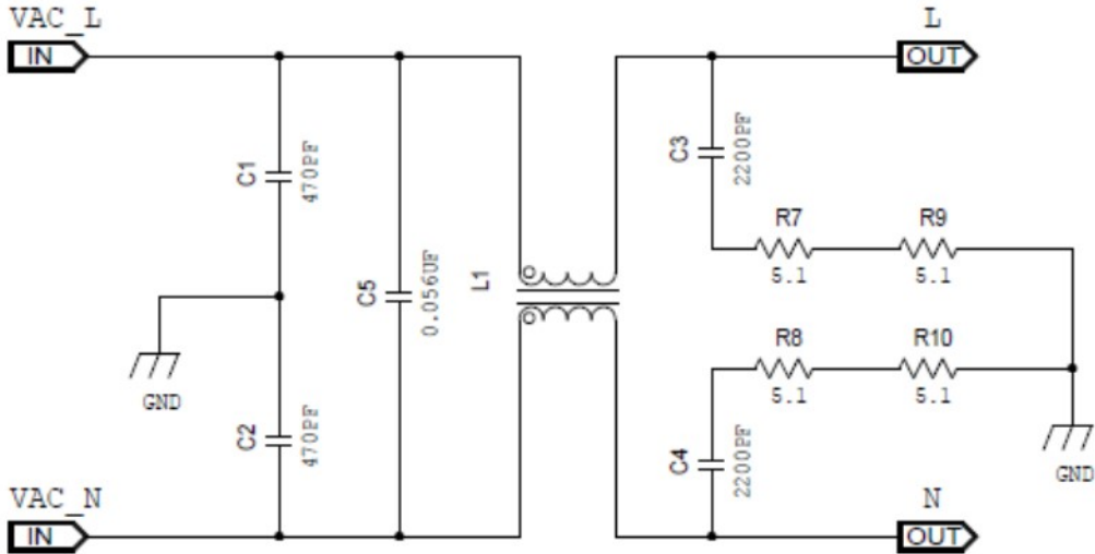
L1: 1.35UH, 3 TURNS, TWO CORES CSC CK270060
