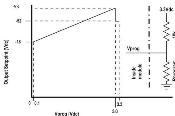
Factory default setting driven by V_{prog}
