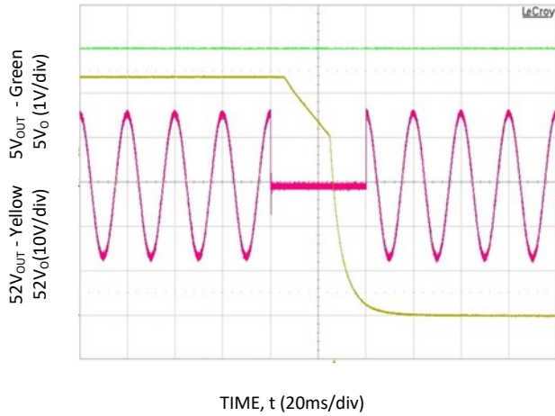
Figure 13. 40ms AC dropout @ full load, V_{IN} = 230V_{AC} .
