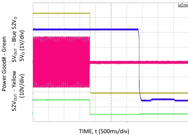
Figure 15. Turn-OFF at full load, V_{IN}=230V_{AC}
