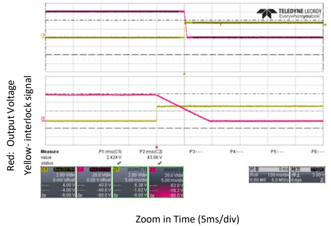
Figure 12. PG# alarmed 10ms prior to V_o < 40V , V_{IN} = 230V_{AC} , Output at Full load
