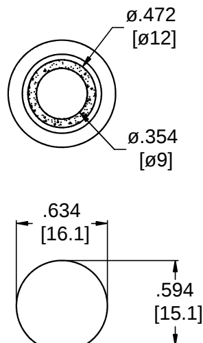
Panel Cutout
