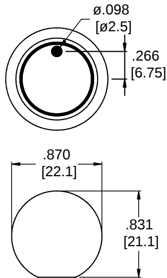
Panel Cutout
