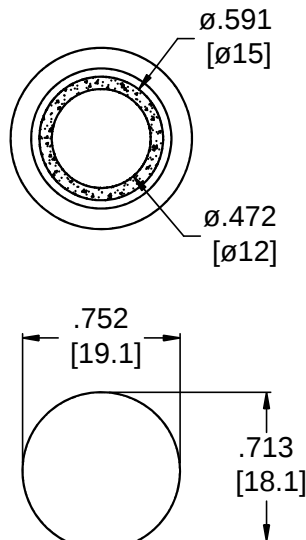
Panel Cutout
