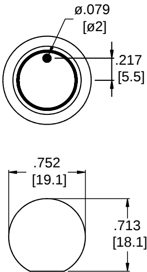
Panel Cutout
