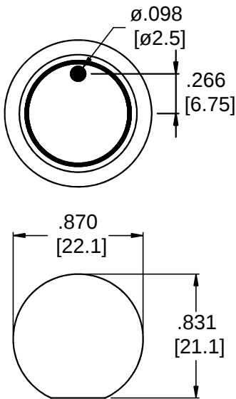
Panel Cutout
