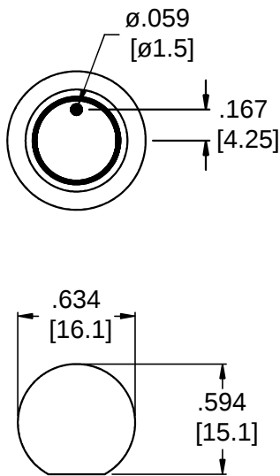
Panel Cutout
